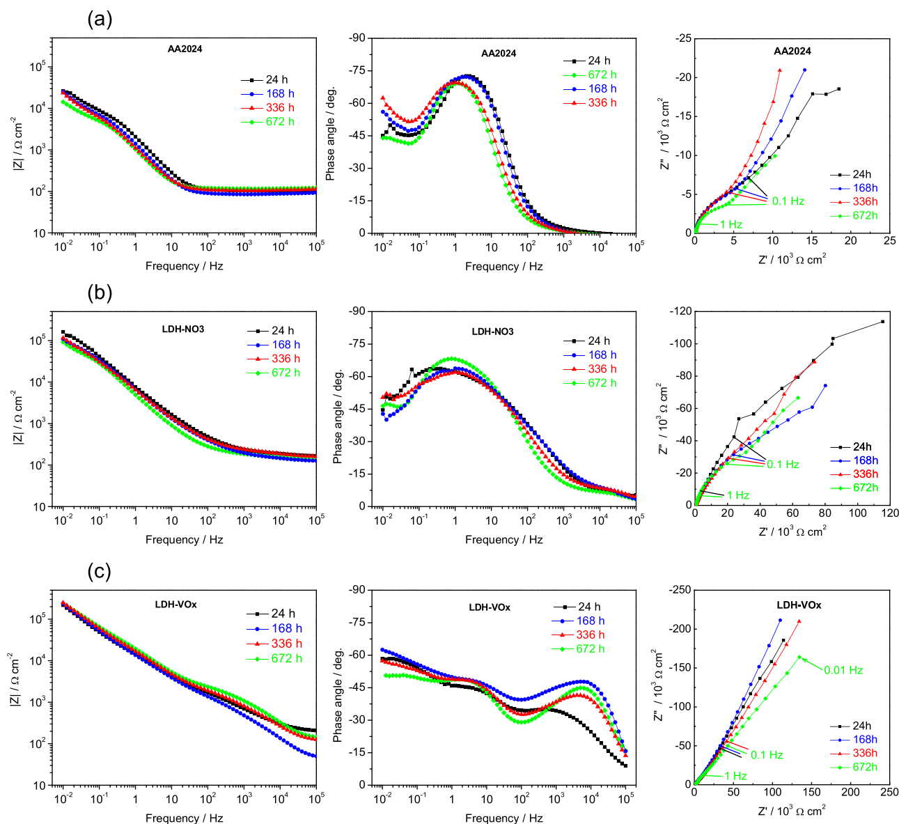
Fig. 3. Bode and Nyquist representations of EIS spectra of AA2024-T3 (a), AA2024-T3 coated with LDH-NO 3 (b) and AA2024-T3 coated with LDH-VO x (c) during immersion in 0.05 M NaCl.
