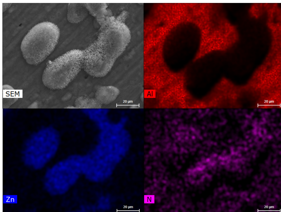
Fig. 2. SEM image of LDH deposited on AA2024-T3 and EDS maps for Al, Zn and N elements.
