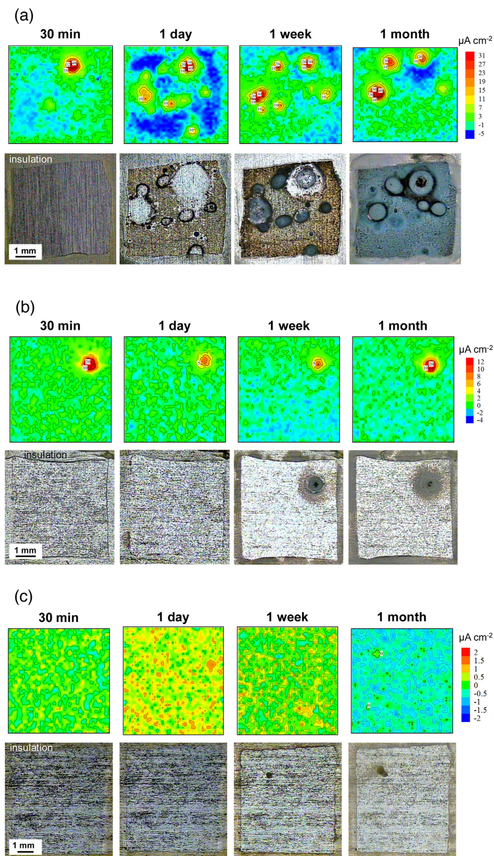
Fig. 6. SVET maps of the AA2024-T3 bare substrate (a), AA2024-T3 coated with LDH-NO 3 and AA2024-T3 coated with LDH-VO x immersed in 0.05 M NaCl. (For interpretation of the references to color in text, the reader is referred to the web version of this article.)
