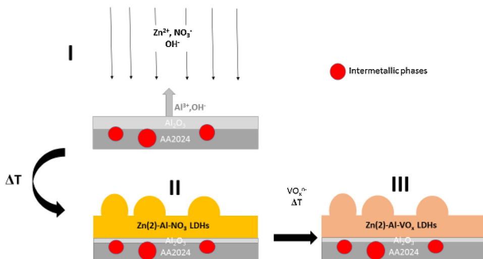
Fig. 1. Scheme of the process for growth of LDH conversion films on AA2024-T3 (according to Ref. [9,11]).
