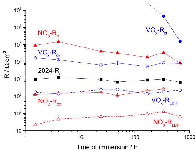
Fig. 5. Evolution of the resistive parameters of the three systems obtained by numerical fitting of the impedance spectra.
