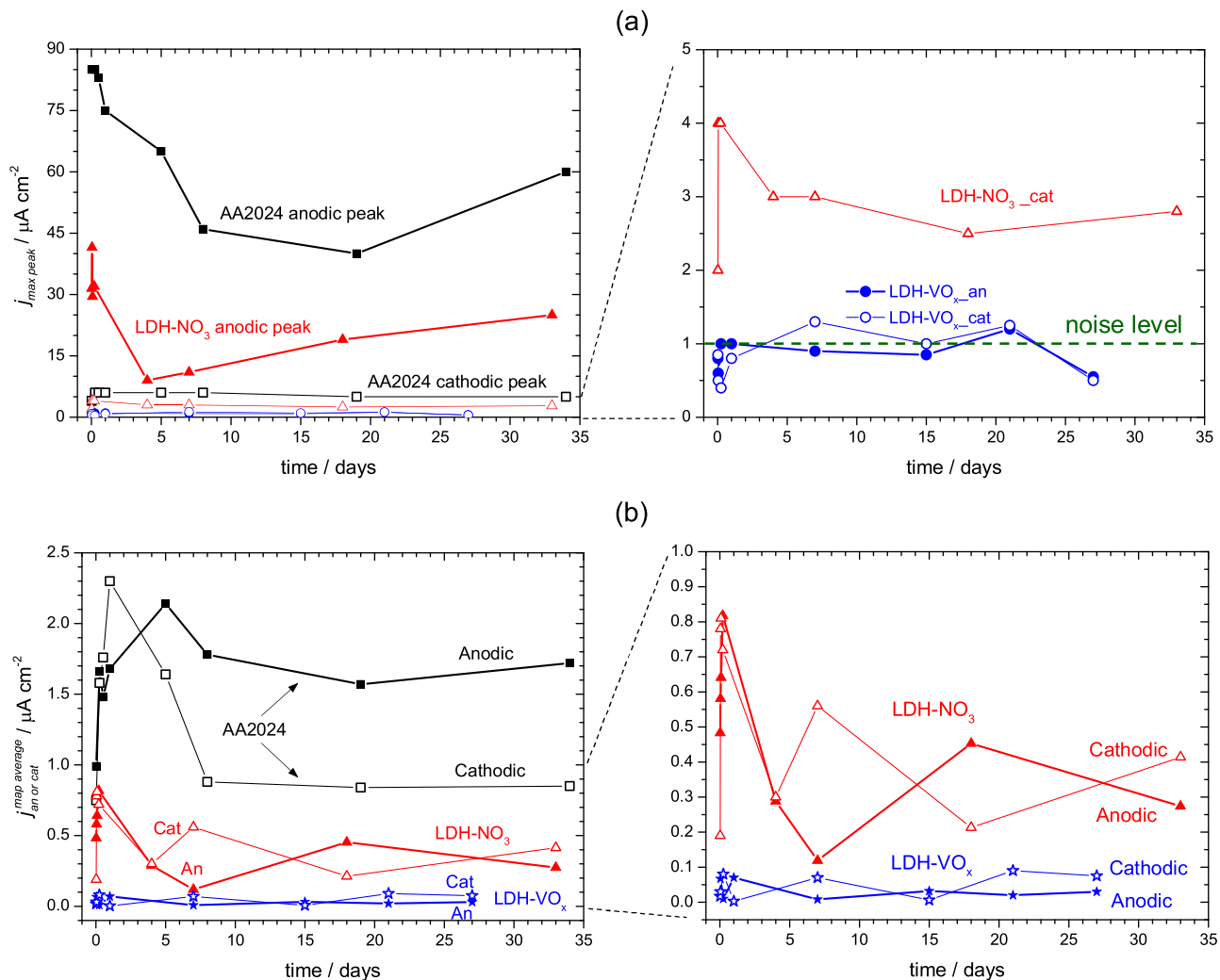
Fig. 10. Plots of highest anodic current density in the SVET maps (maximum peak height) (a) and the average current density in the map (b) for AA2024-T3, LDH-NO 3 and LDH-VO x .
