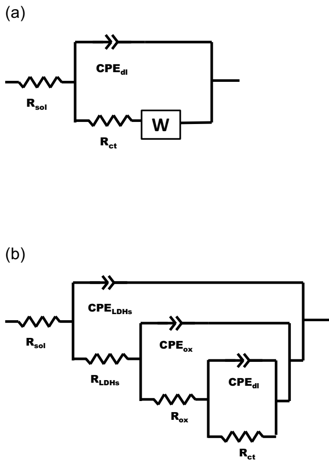
Fig. 4. Equivalent electric circuits used to fit the EIS spectra.
