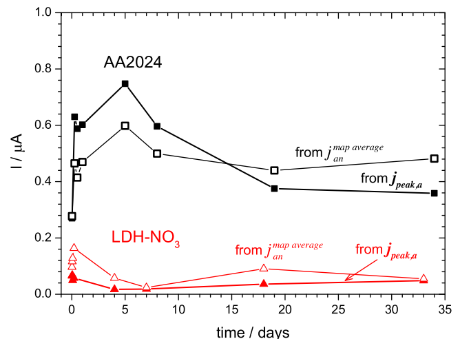
Fig. 11. Total current in sample estimated by SVET.
