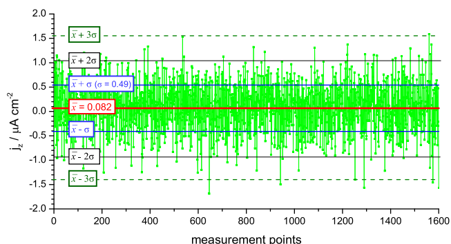
Fig. 9. Noise level of measurements in 0.05 M NaCl performed in a Petri dish with no sources of current present. Shown are the mean current ( \bar{x} ), the standard deviation ( \sigma ), 2\sigma and 3\sigma .
