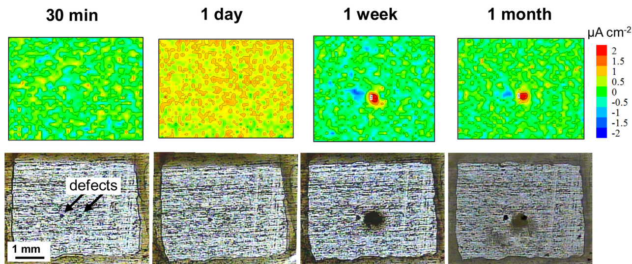
Fig. 8. SVET maps and optical photographs of a sample of AA2024-T3 coated with LDH-VO x , with two pin-hole defects.
