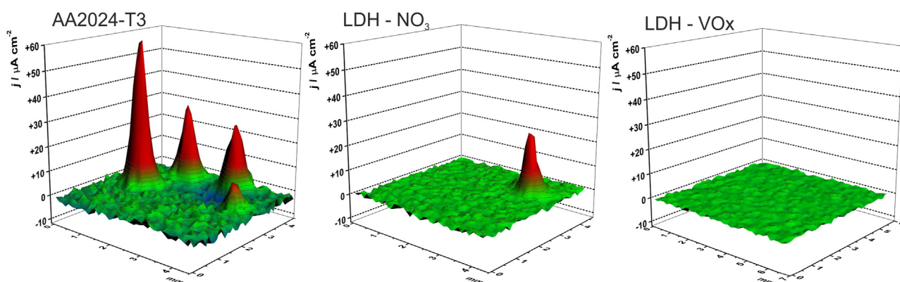
Fig. 7. (A) 3D SVET maps of the different systems after 1 month of immersion in 0.05 M NaCl.
